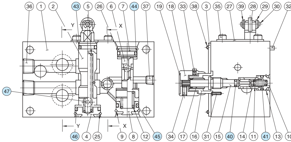
Section X-X
